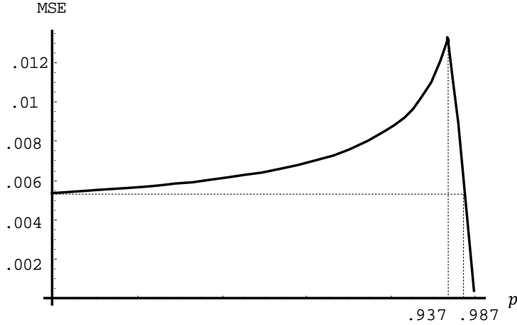
Fig. 3. Mean-square error in the two-sender game with uniform priors, c_A = .2 , c_B = 0 , p_A = 1 , and p_B = p .
