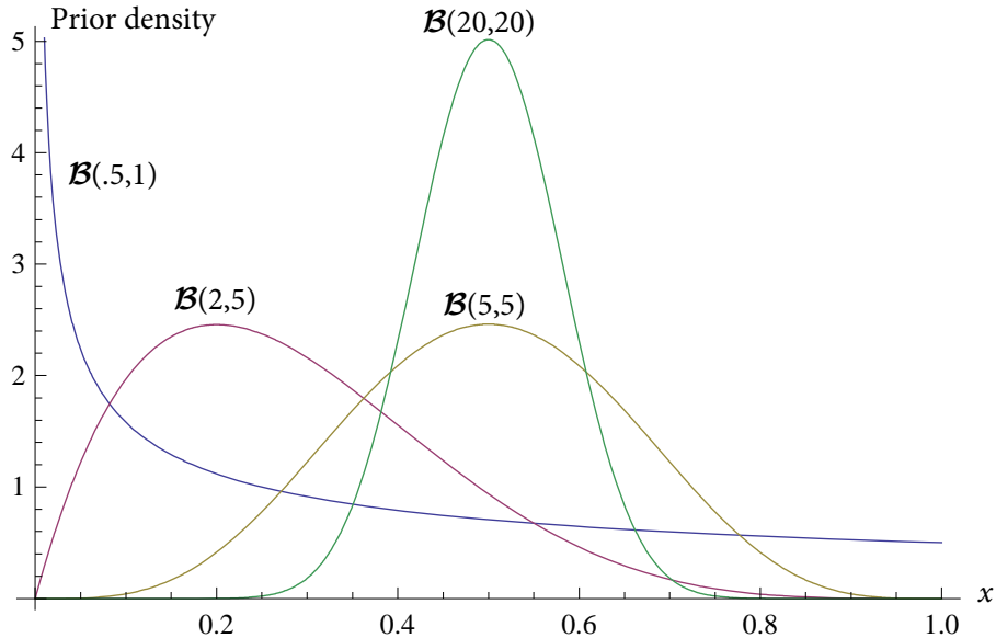
Fig. 2. Some of the Beta distributions used in Table 1
