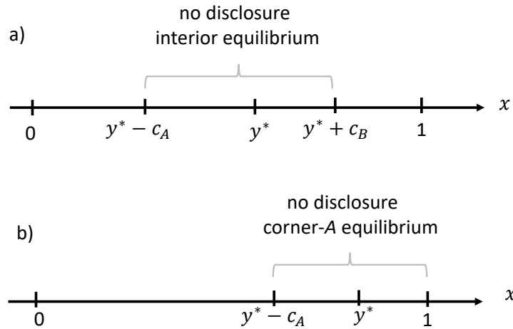
Fig. 1. Interior and corner equilibria
